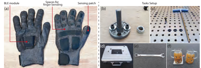
Fig. 1. Tactile sensing gloves (a) and target tasks setup (b-f). Tasks are hand tightening a bolt (b), using a T-handle screwdriver (c), opening a case (d), reorienting a wrench (e), and pouring a pitcher (f).
