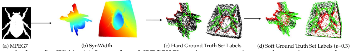
Fig. 3: Example from SynWidth. (a) Image from MPEG7[27] used to generate inner and outer intercepts for width mate generation. (b) Generated point clouds and meshes. (c) Downsampled point clouds at training and inference time, along with ground truth set correspondences denoted in red and green. (d) Soft set correspondences by relaxing the constraint of distance to ground truth correspondences. The tolerance \epsilon is set to 0.3 for visualization purpose. Actual training procedure uses \epsilon = 0.1 .
